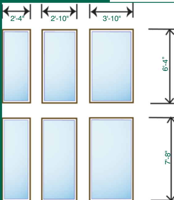
Figure 5-12: Patio door replacement unit sizes
